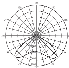
PSL 07 100w
